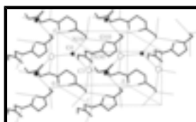
Fig. 2. Packing diagram of (I). Side chains of amino acids are omitted for clarity. Dotted lines represent hydrogen bonds. Circles and filled-circles represent chloride ion (Cl) and water (O1) molecules.
