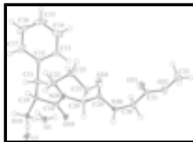
Fig. 1. A view of (I) with displacement ellipsoids drawn at the 50% probability level with the aid of PLATON (Spek, 2003). Dotted lines represent hydrogen bonds.
